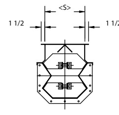
SECTION C-C LOW PROFILE STYLE INLET
