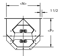
SECTION A-A BY-PASS STYLE INLET
